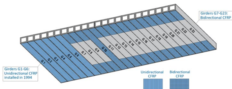
Figure 92. Foulk Road bridge-plan of repaired girders.
