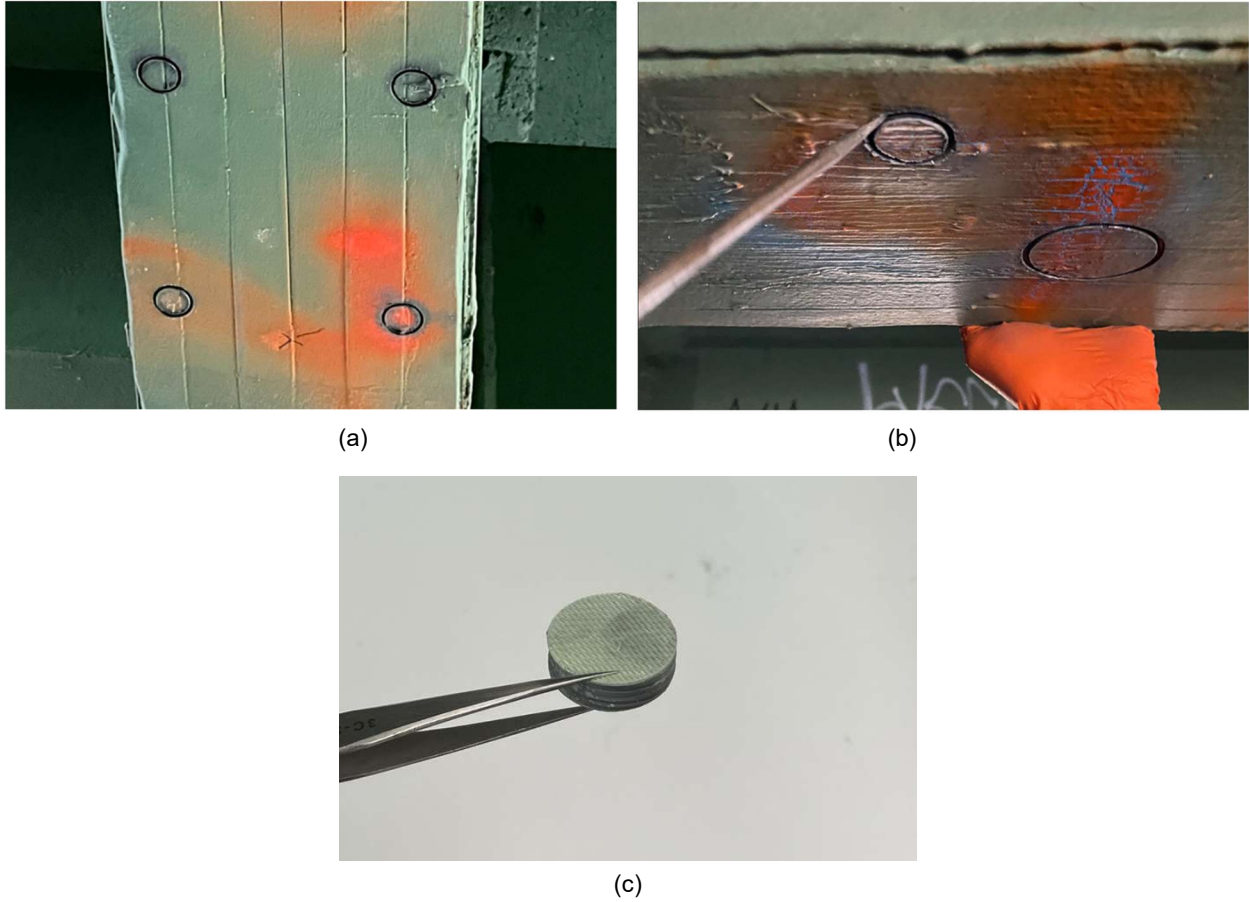
Figure 65. CFRP sample collection at Br 1-704: (a) CFRP composite drilled using a 1-1/8-in. diamond-coated core saw, (b) sample collection under progress using flat-head screwdriver, and (c) 1-in.-diameter CFRP sample.
