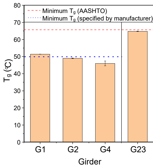
Figure 100. Glass transition temperature measured on samples from girders G1, G2, G4, and G23.
