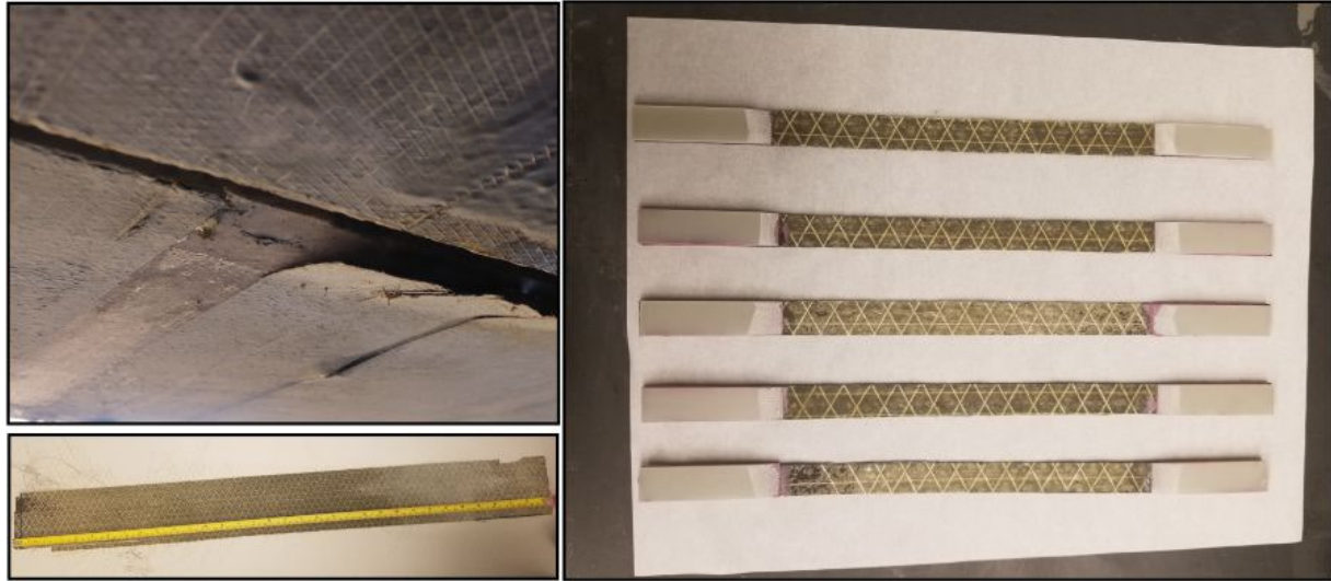
Figure 94. Specimens for tensile testing were prepared using CFRP material extracted from G1.
