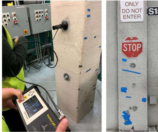
Figure 23. An example of the bond pull-off test setup.
